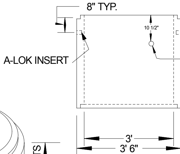
MODEL WT3 - 3' TALL
