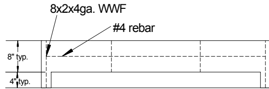
26" x 26" opening
